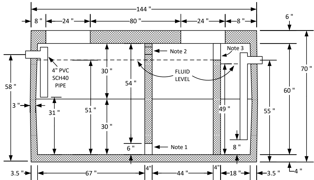
SIDE SEC.
